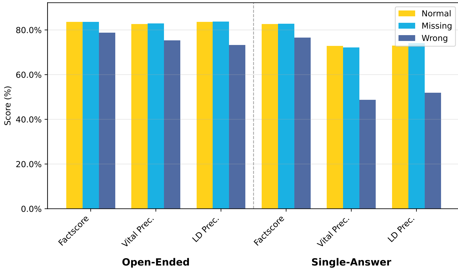
Precision Metrics
